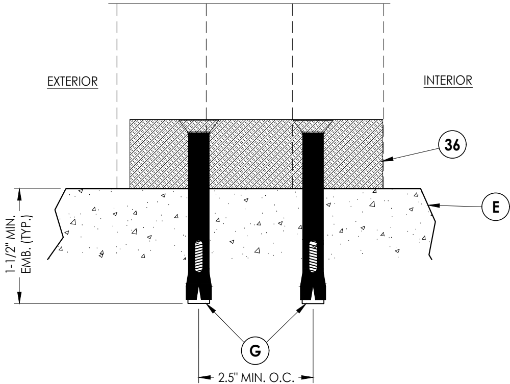
2 5 VERTICAL CROSS SECTION @ Removable Mullion
