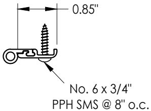
6 WEATHERSTRIP NGP 137N
