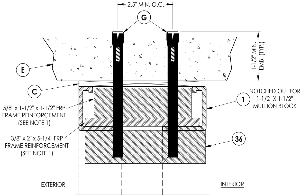
1 5 VERTICAL CROSS SECTION @ Removable Mullion
