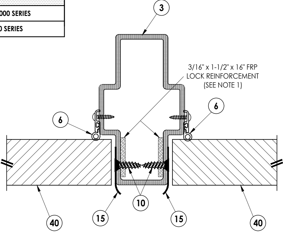
2/3 HORIZONTAL CROSS SECTION Outswing configuration
