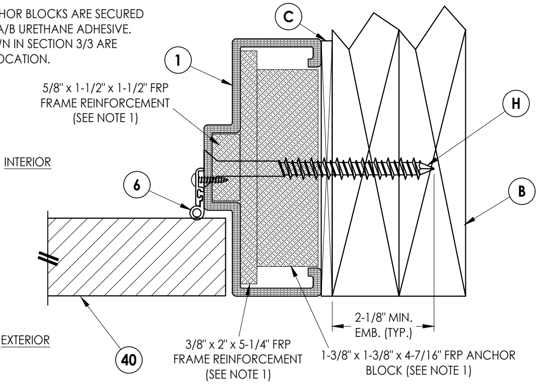
3/3 HORIZONTAL CROSS SECTION Outswing configuration
